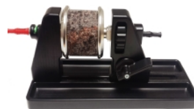
IP/Resistivity Pad with KT-20 IP Sample Holder
